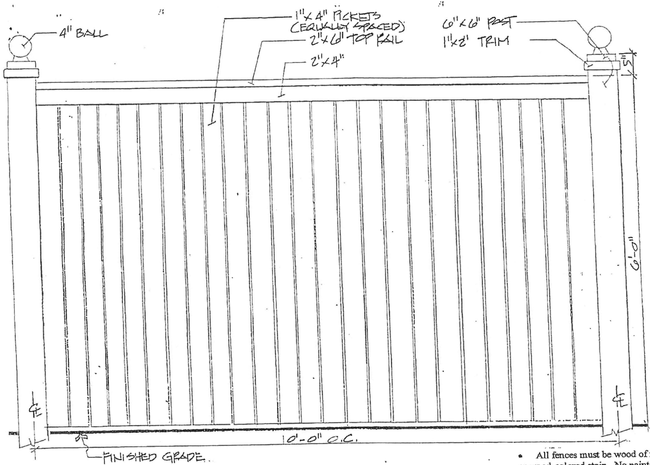
Fence Design #1 Not to Scale
